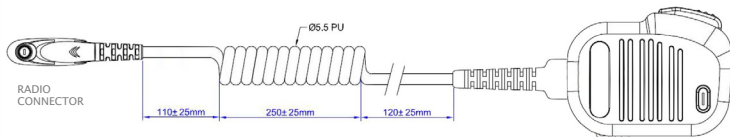
LINE DIAGRAM—DIMENSIONS
