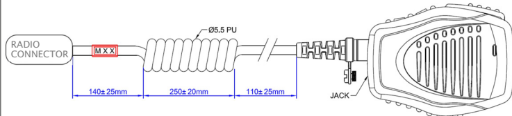
LINE DIAGRAM—DIMENSIONS
